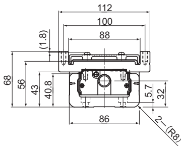
B-B cross section
