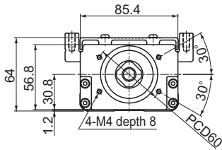
A arrow view
