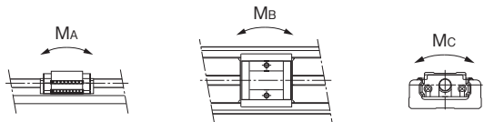
With a single short type block (Model SKR-C)
