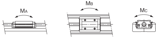
With a single long type block (Model SKR-A)
